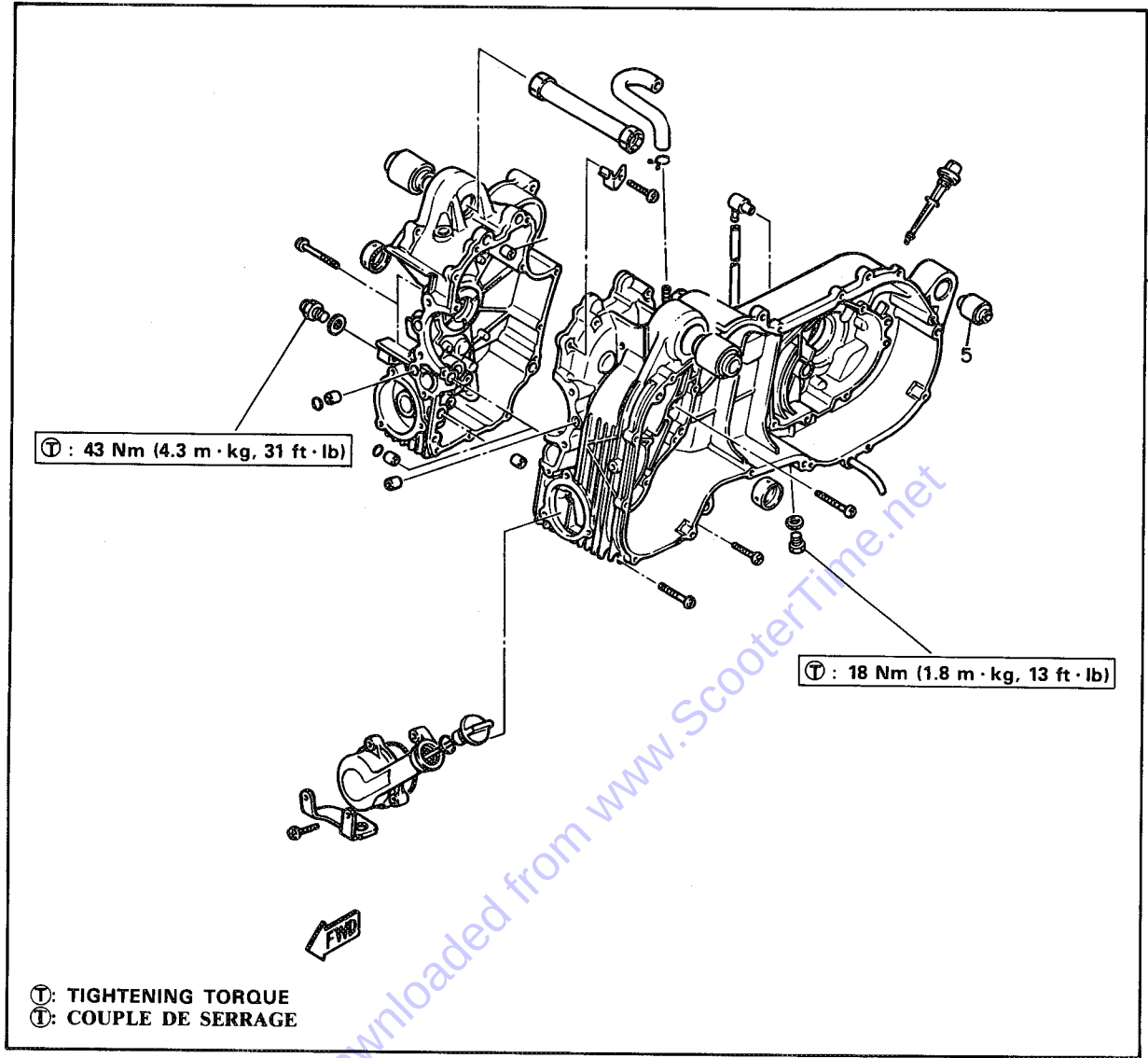
CRANKCASE (LEFT) CARTER (GAUCHE)
