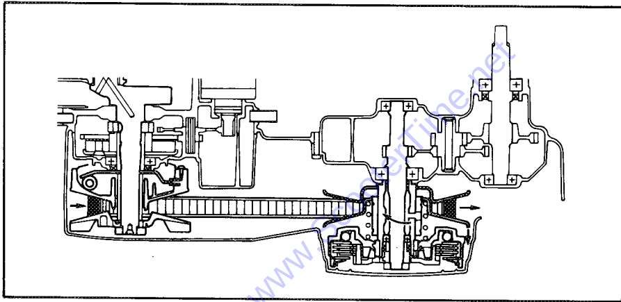
Route of engine power
