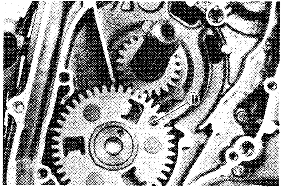
1. Knock pin
