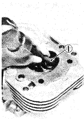
1. Valve guide remover 2. Valve guide installer
