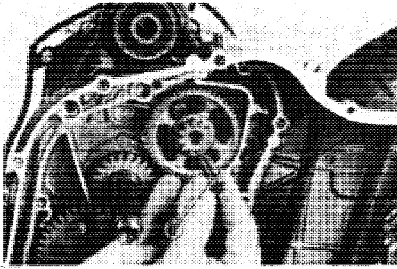
1. Idle gear shaft
