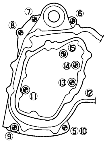
CRANKCASE (LEFT) CARTER (GAUCHE)
