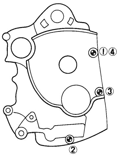
CRANKCASE (RIGHT) CARTER (DROIT)
