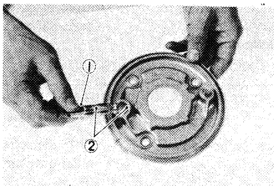
1. Camshaft 2. Apply grease
