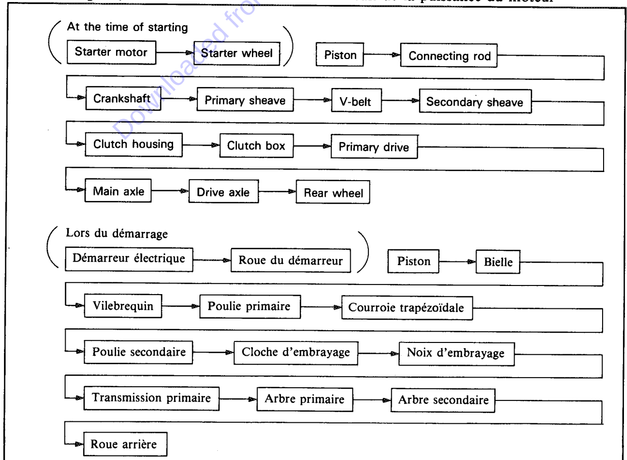
Route of engine power
