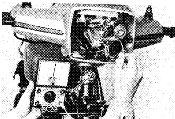
1. Br/W 2. Ground
