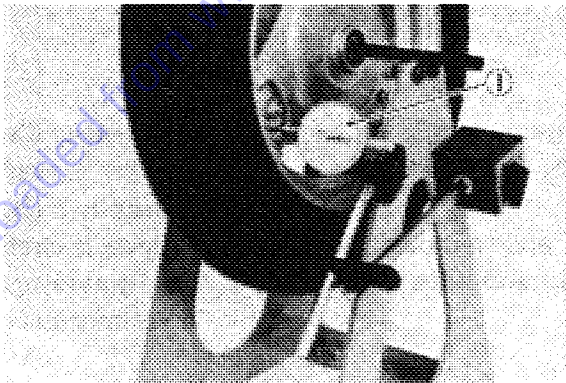
1. Dial gauge
