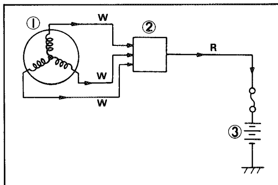
1. Generating coil (Stator coil) 2. Silicon rectifier 3. Battery
