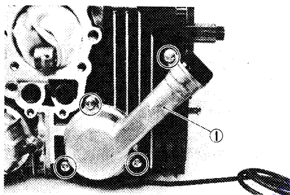
1. Oil filler
