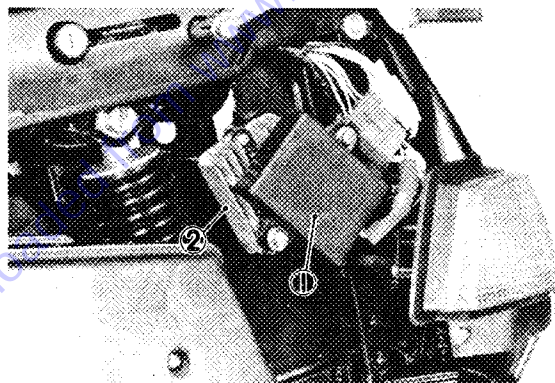
1. Ignitor unit 2. Voltage regulator/ Rectifier
