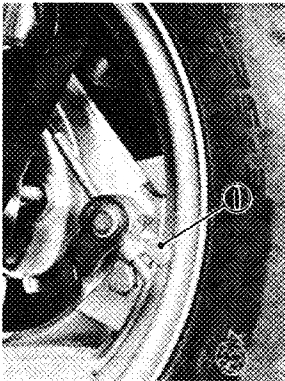
1. Adjuster a. Free play 5 ~ 15 mm (0.2 ~ 0.6 in)
