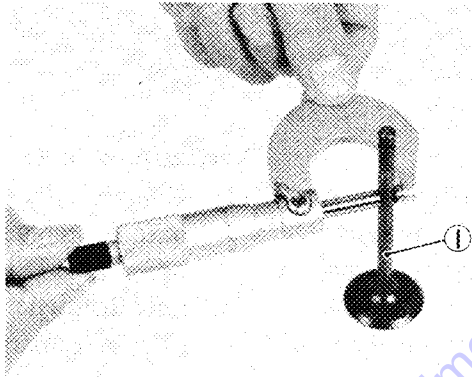
1. Valve
