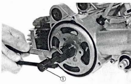
1. Flywheel puller
